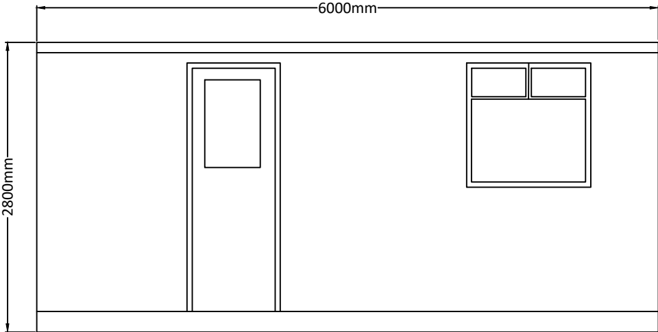
FRONT ELEVATION
